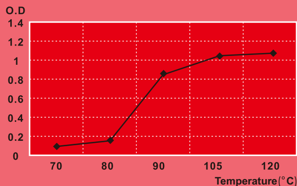
STATIC SENSITIVITY
