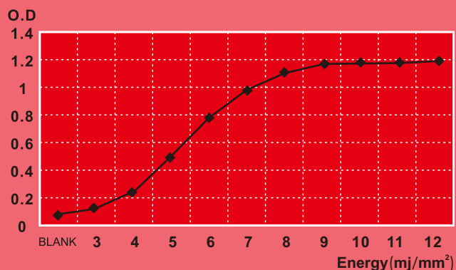
DYNAMIC SENSITIVITY
